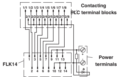
PLC-V8L/FLK14/OUT connection scheme
